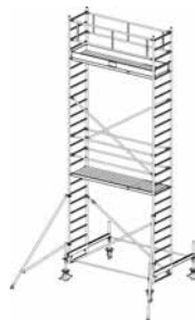
Working height: 7.40 m Scaffold height: 6.40 m Platform height: 5.40 m
