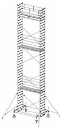
Working height: 11.40 m Scaffold height: 10.40 m Platform height: 9.40 m
