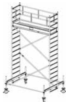
Working height: 5.40 m Scaffold height: 4.40 m Platform height: 3.40 m
