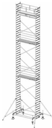
Working height: 13.40 m Scaffold height: 12.40 m Platform height: 11.40 m
