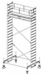
Working height: 6.40 m Scaffold height: 5.40 m Platform height: 4.40 m
